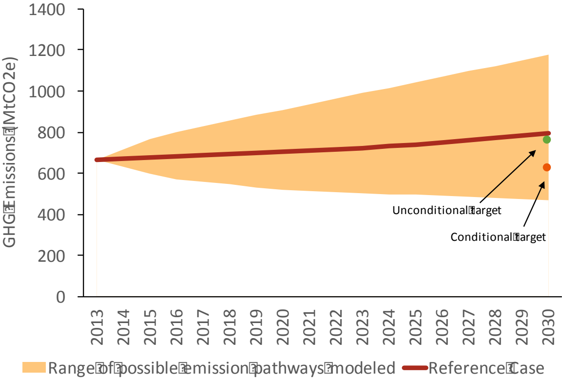
Figure 4: Range of Reference Case Emissions
