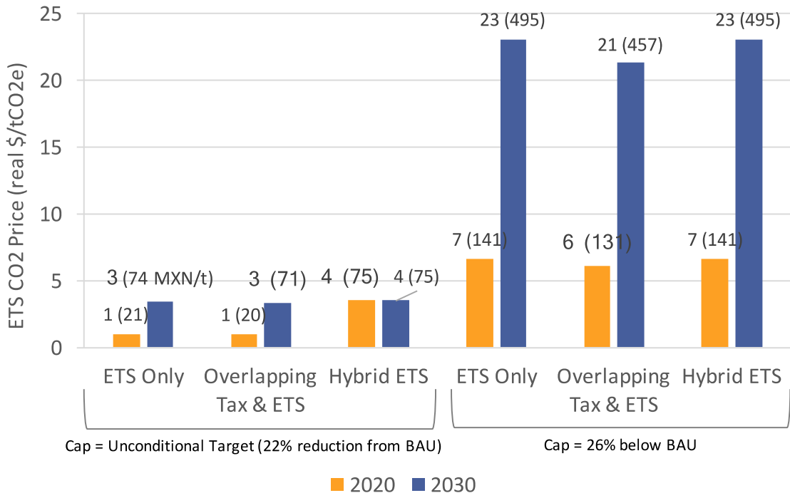
Figure 5: ETS Carbon Prices by Scenario
