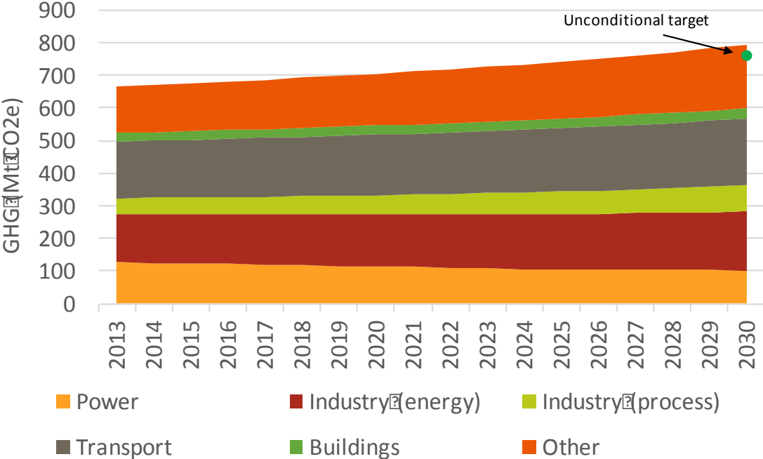
Figure 3: Reference Case Emission Projections by Sector
