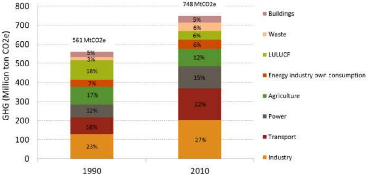
Figure 1: GHG Emissions by Sector, 1990 and 2010
